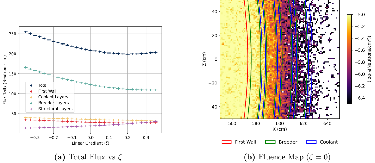
Figure 7: (a) Neutron track length tally within reactor components, paired with a heatmap of neutron fluence depletion through the reactor wall (b).
